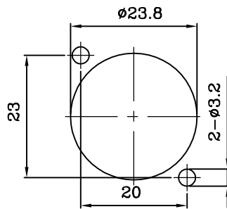
Panel cut out (front side)
