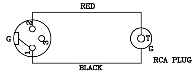
XLR FEMALE
